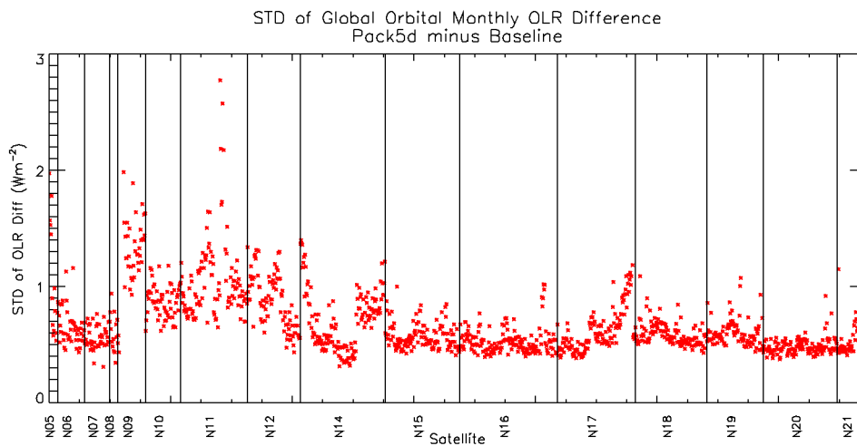
Figure 6 Similar to Figure 5 but is for the standard deviation of the global monthly mean OLR differences.
