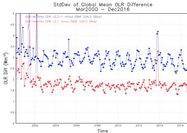
Figure 8 Similar to Figure 7 but for the standard deviation. The OLR CDR v02r07 has improved significantly in both the annual cycle amplitude as well the spatial distribution, relative to the EBAF Ed4 data. The standard deviation of the regional differences in the two products is below 2 \text{ Wm}^{-2} . The spikes shown in the earlier period and one near 2014 are due to the sampling differences, mostly due to the missing data in MODIS that prevents CERES from generating products.
