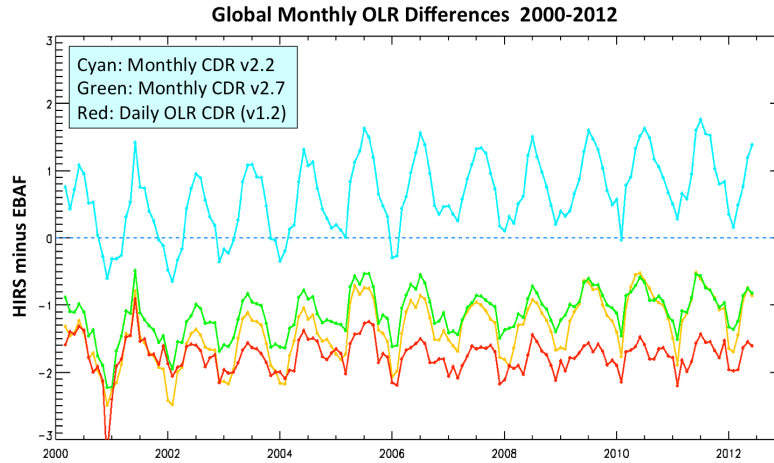
Figure 17 Comparison of OLR CDR (Monthly v2.2, v2.7 and Daily v1.2) products against CERES EBAF v2.6r OLR product.
