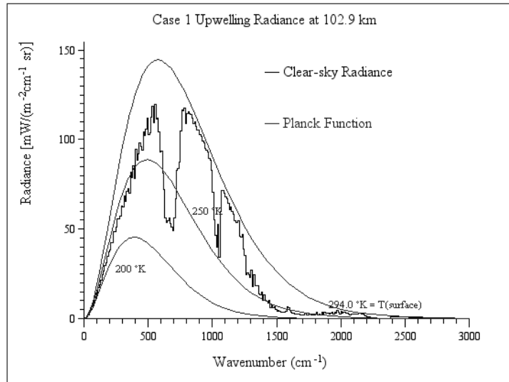
Figure 4 TOA upward longwave radiation spectrum for standard mid-latitude summer case. The smooth curves are the Planck function evaluated at 200°K, 250°K and 294°K (surface temperature for this case), respectively for reference purpose.
