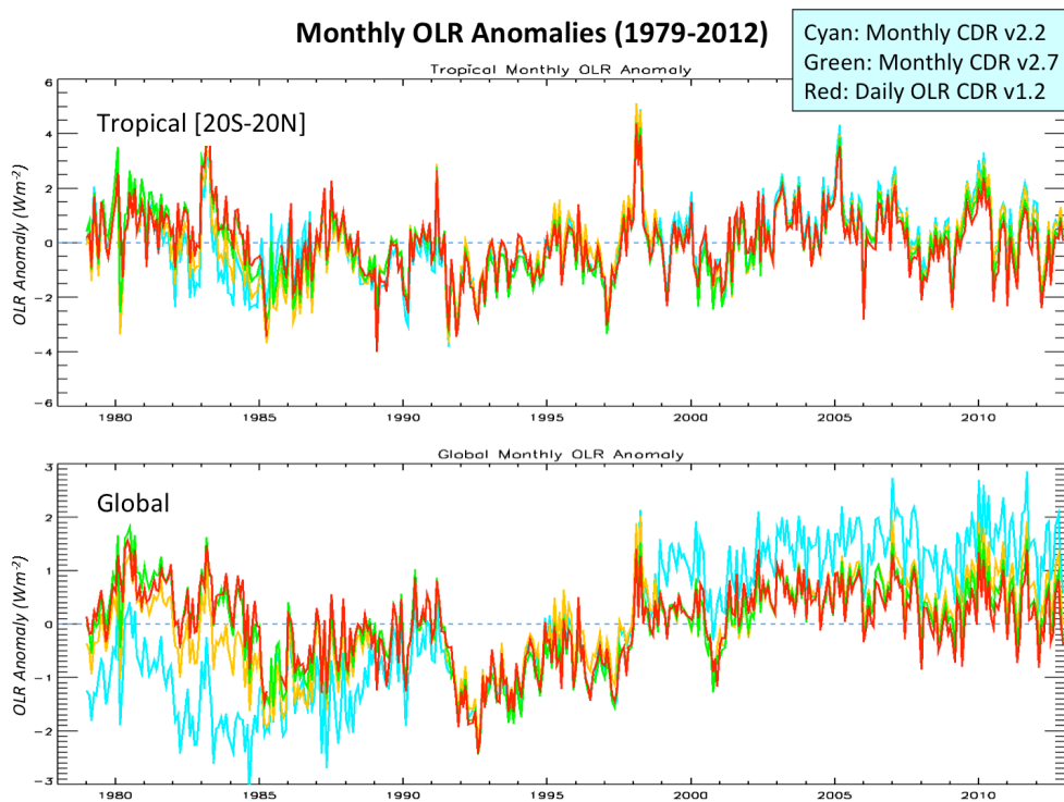
Figure 16 Comparison Tropical and Global OLR Anomalies of OLR CDR products (Monthly v2.2, v2.7 and Daily v1.2).
