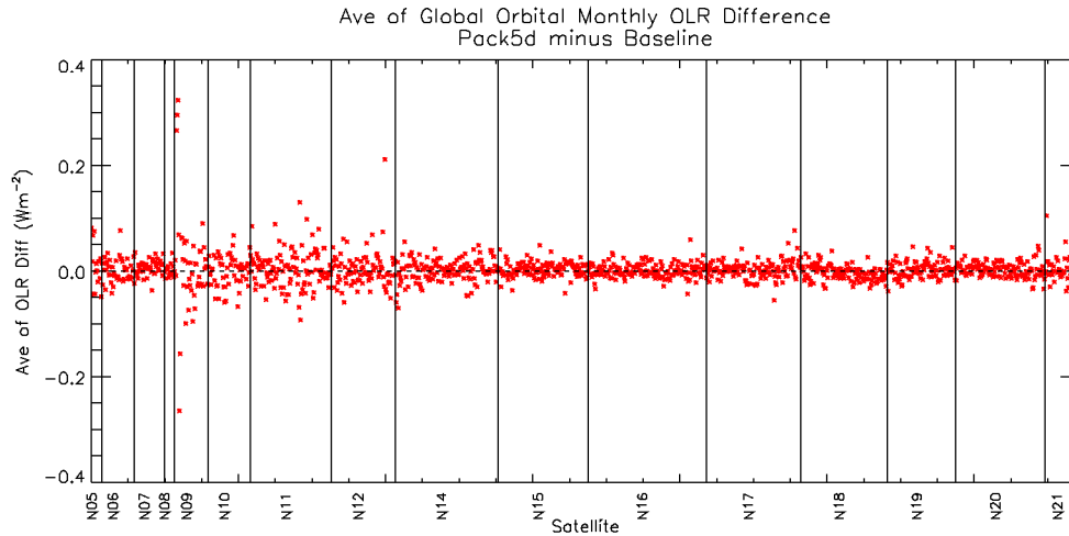
Figure 5 Differences of Global mean OLR CDR between the Rejuvenated and the baseline version of the v02r07 code packages. (Rejuvenated version is labeled as “Pack5d”)
