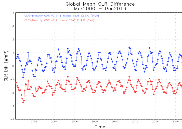
Figure 7 Time series of the global mean monthly OLR, OLR CDR minus EBAF. (Blue: OLR CDR v02r02-1; Red: v02r07) The smaller disagreement in the annual cycle discrepancies is an evidence of the improvements in v02r07. Note that the EBAF Ed.4 OLR has been adjusted upwards by an about 0.5 \text{ Wm}^{-2} relative to Ed2.8. The trended differences between 2000-2003 are related to the relatively larger uncertainties in the EBAF data that was constructed with TERRA CERES observations only.
