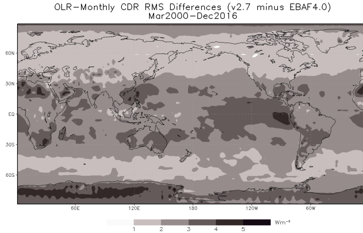
Figure 13 Similar to Figure 11 but is for the RMS differences. The relatively larger discrepancies were found over the eastern tropical Pacific Ocean, Sahara deserts, and the eastern Antarctica.
