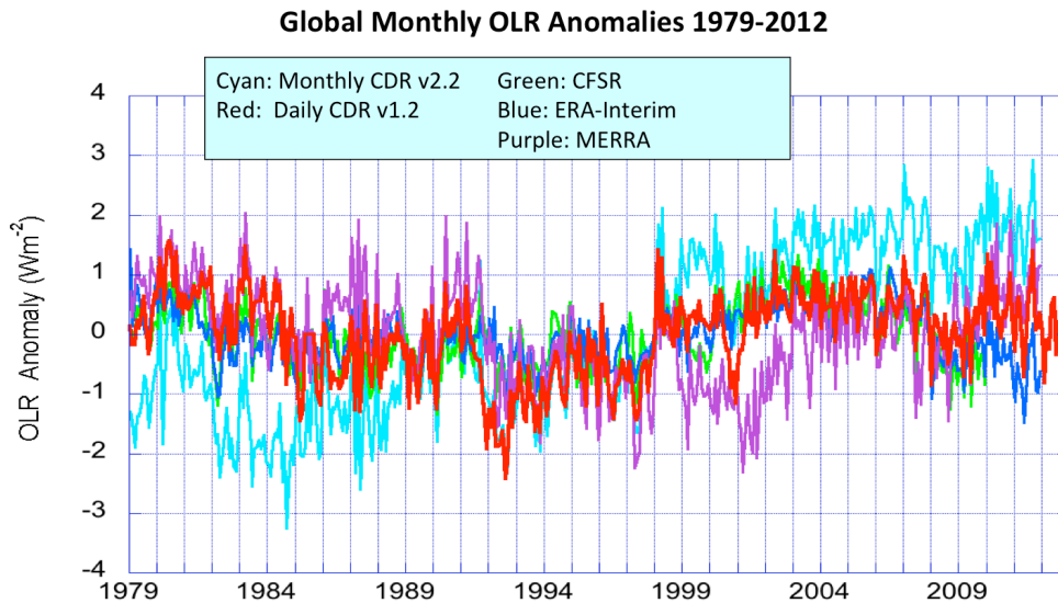
Figure 18 Comparison of OLR CDR (Monthly v2.2, and Daily v1.2) products with Reanalysis data sets, CFSR, ERA-Interim and MERRA.
