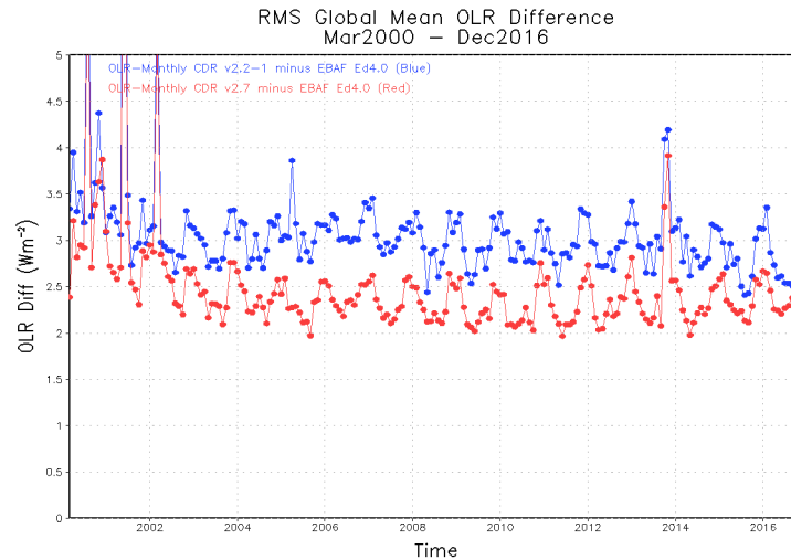
Figure 9 Similar to Figure 7 but for the RMS differences. The OLR CDR v02r07 has improved the overall agreement of the spatial distribution, relative to the EBAF Ed4 data. The RMS of the regional differences in the two products is at about 2.5 \text{ Wm}^{-2} level.
